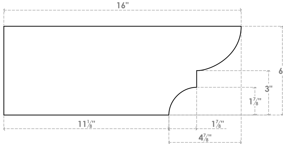
SIDE PROFILE
